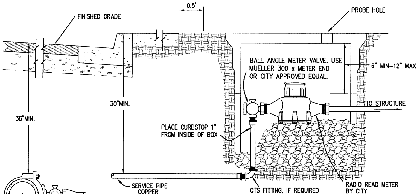
CORPORATION STOP— MUELLER 300 BALL VALVE OR CITY APPROVED EQUAL
