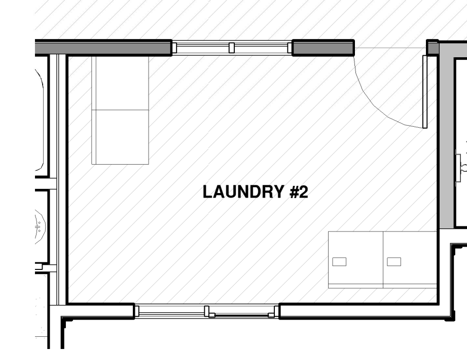
③ LAUNDRY - 3RD FLOOR 1/4" = 1'-0"
