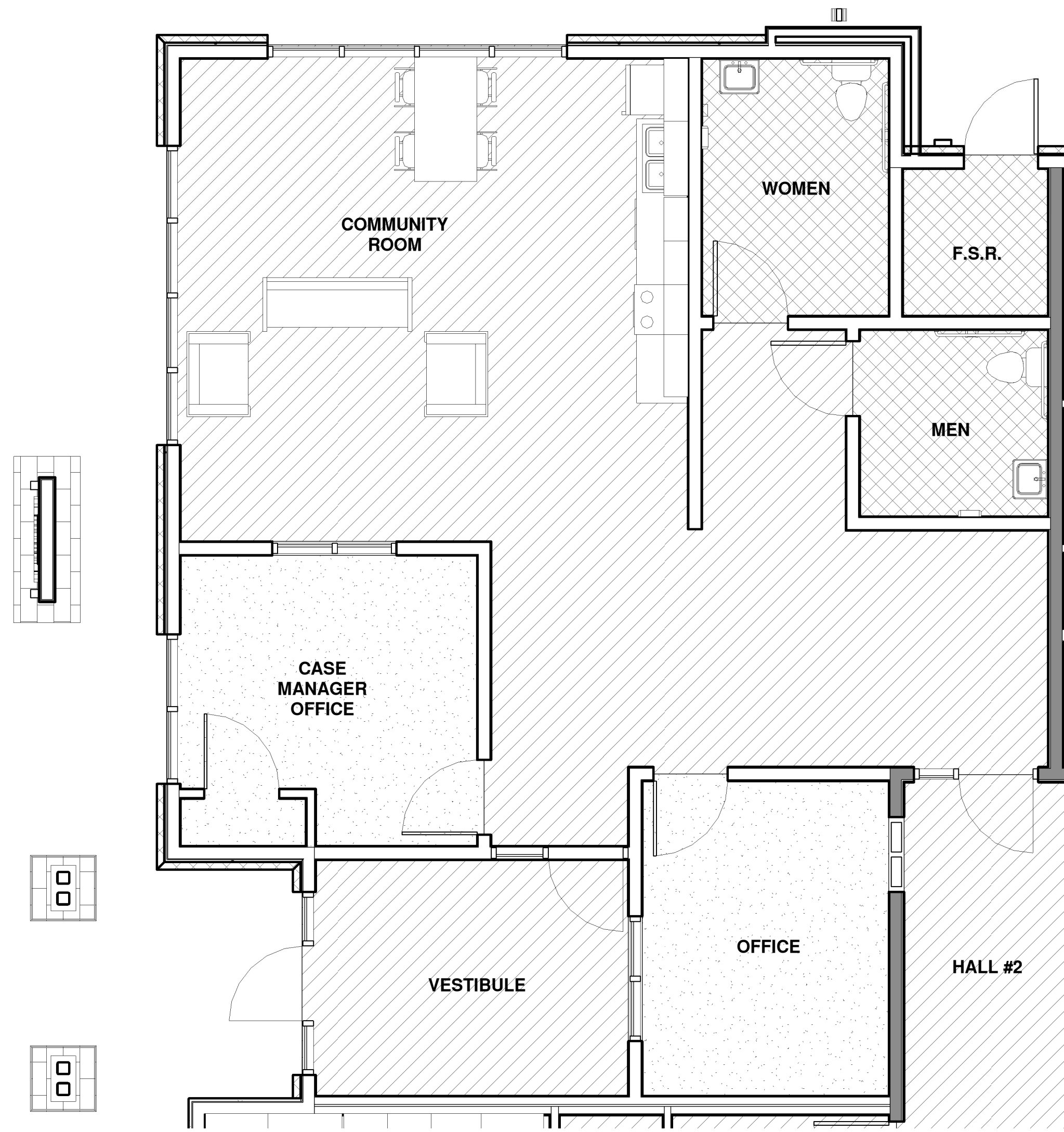
① COMMUNITY CENTER PLAN 1/4" = 1'-0"
