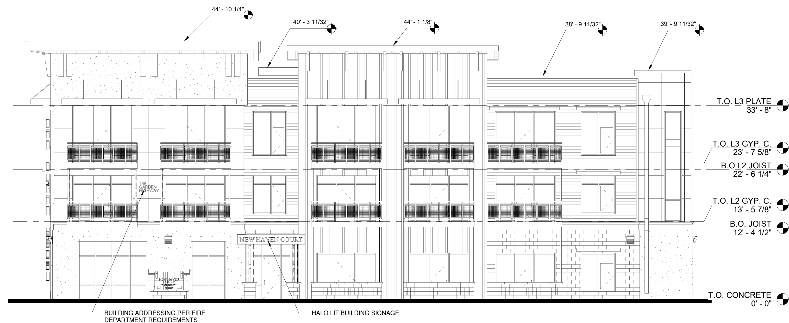
① WEST ELEVATION 1/8" = 1'-0"
